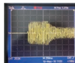
Flying start motor/network waveform
